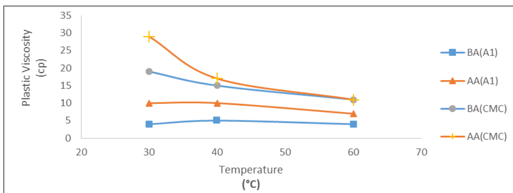
Fig 3: Plastic viscosity of Mud samples before and after aging against temperature
