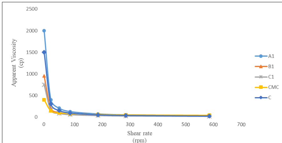
Fig 2: Apparent viscosity of Mud samples at different shear rates after aging at 30°C
