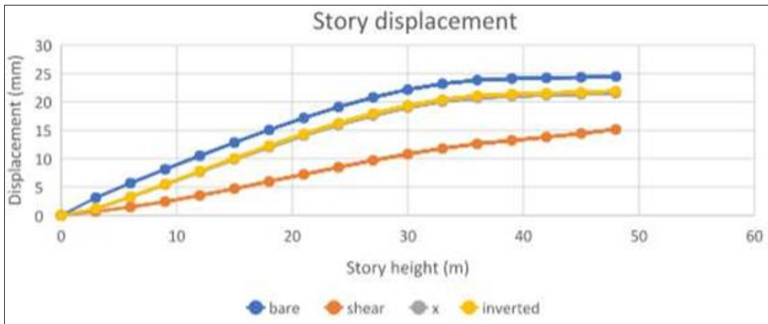
Fig 6: Comparative Graph Showing Displacement in Y Direction
