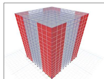
Fig 5: Building with Shear Wall
