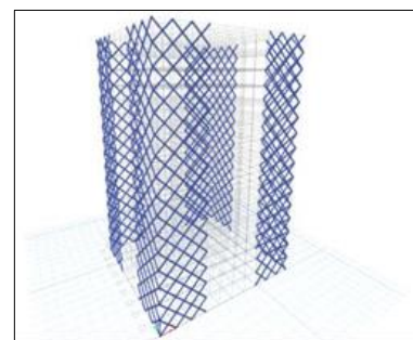
Fig 4: Building with Inverted V Bracing
