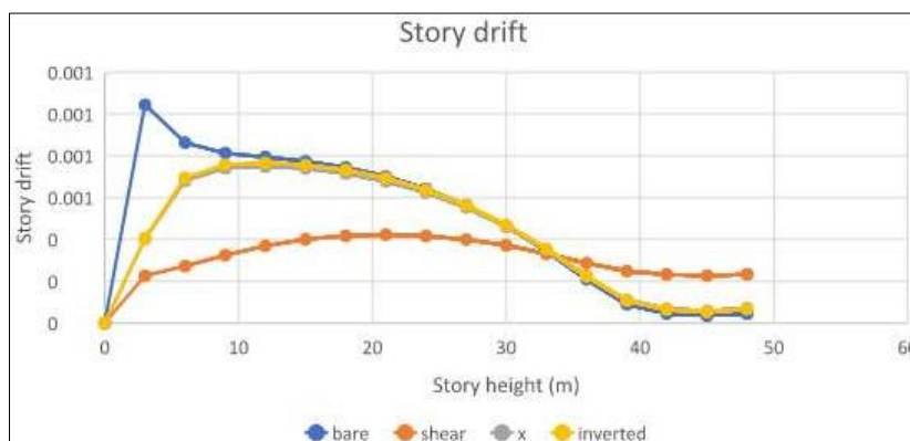
Fig 7: Comparative Graph Showing Displacement in Y Direction
